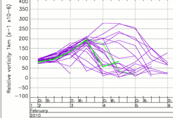
Feature-specific plume of relative vorticity
