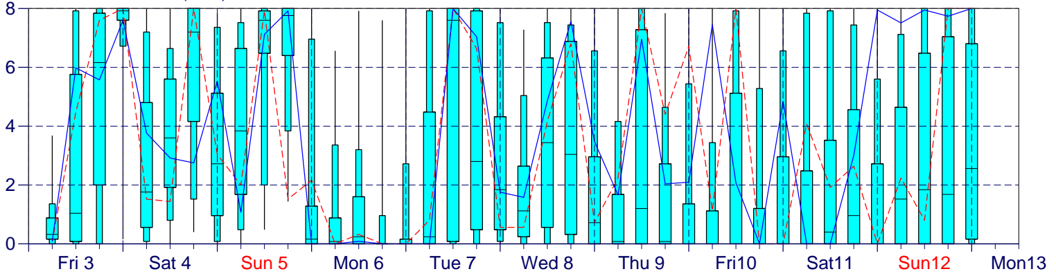
Total Precipitation (mm/6h) 65 41
