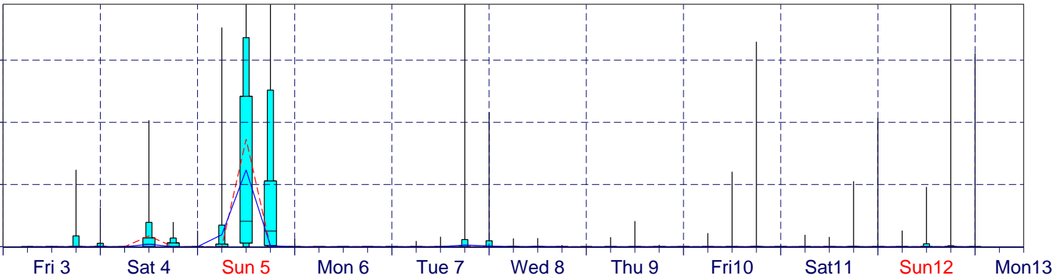
Total Precipitation (mm/6h) 37 10
