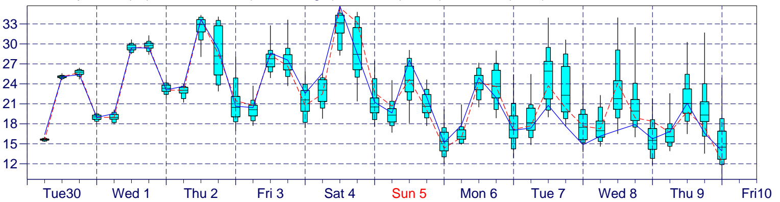
2m Temperature(°C) reduced to 2 m (station height) from 6 m (T1279) and 11 m (T639)
