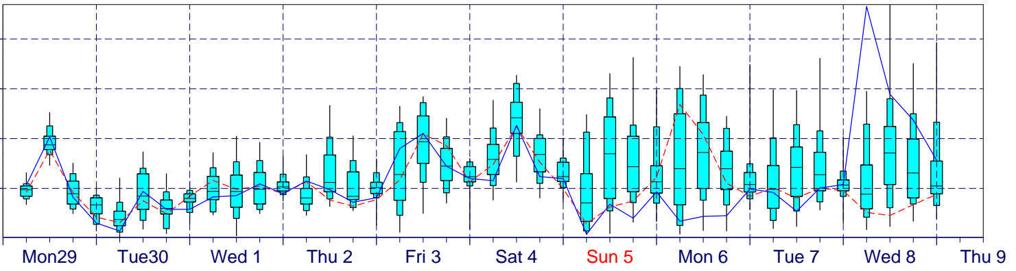
2m Temperature(°C) reduced to 164 m (station height) from 203 m (T1279) and 218 m (T639)
