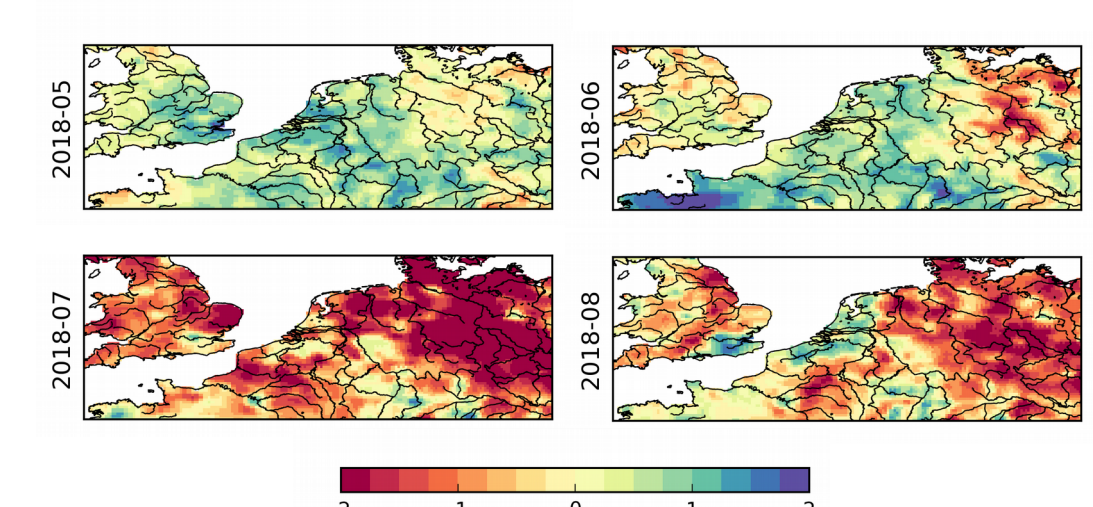
Figure 4: SWI monthly anomalies (scaled by stdev) over 2008-2018 for May to August 2018
