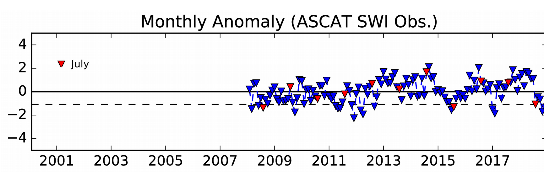
Figure 5: Monthly Anomaly time-series (scaled by the standard deviation) of satellite derived ASCAT SWI over 2008-2018. Months of July are highlighted in red, straight dashed lines represent values for July 2018.
