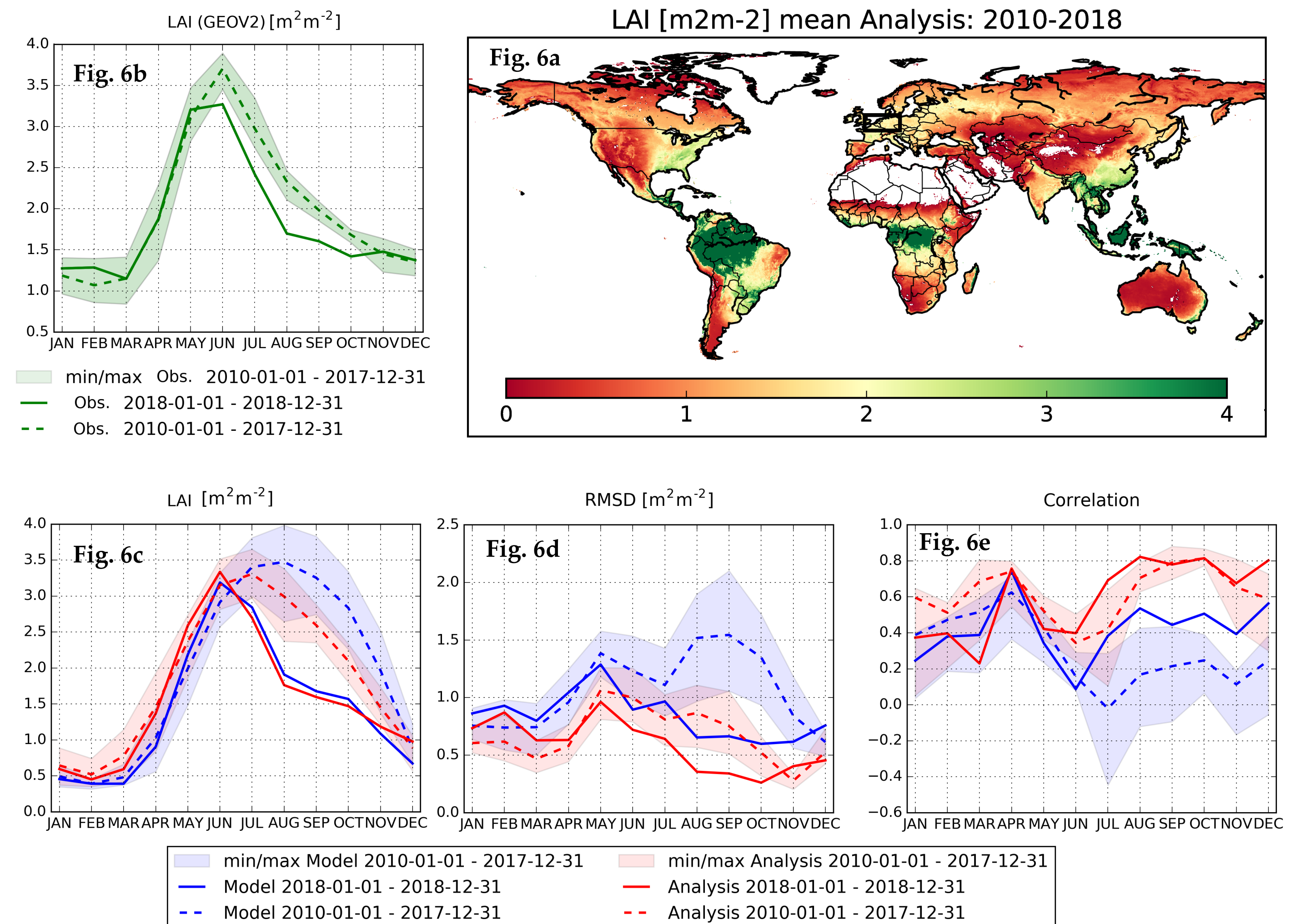
Figure 6: a) Global reanalysis of LAI from LDAS-Monde averaged over 2010-2018 ( 0.25^\circ \times 0.25^\circ ). b) Satellite derived LAI seasonal cycle averaged over 2010-2017 (dashed line) and for the year 2018 and the domain presented in figure 2. c) Same as b) for LAI from LDAS-Monde open-loop, i.e. no assimilation, (in blue) and LDAS-Monde analysis (in red). d) Seasonal RMSD values between LAI from the model (in blue) and the analysis (in red) and the observations for 2010-2017 (dashed line) and 2018 (solid line). e) Same as d) for correlations values.
