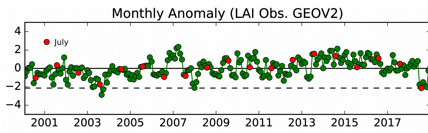
Figure 3: Monthly Anomaly time-series (scaled by the standard deviation) of satellite derived GEOV2 Leaf Area Index over 2000-2018. Months of July are highlighted in red, straight dashed lines represent values for July 2018.
