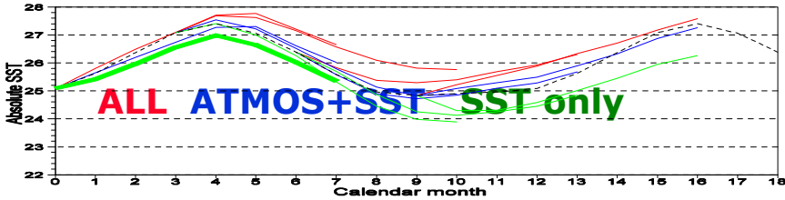
NINO3 mean absolute SST
