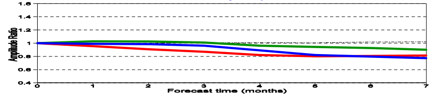
NINO3 SST anomaly amplitude ratio
