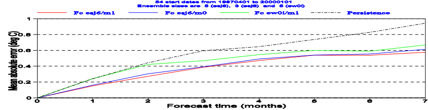
NINO3 SST mean absolute errors
