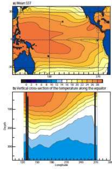
Figure 4: Mean of the reanalysis for 1983 to 1996
