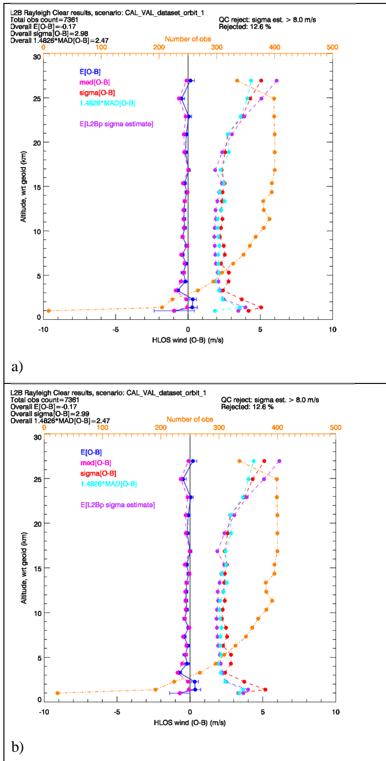
Figure 8. Aeolus L2B Rayleigh-clear verification statistics shown with varying altitude for a) with dynamic p, T derived altitudes and b) with fixed height = 0.49. Simulation is one orbit of 320 km realistic ECMWF model derived E2S inputs.
