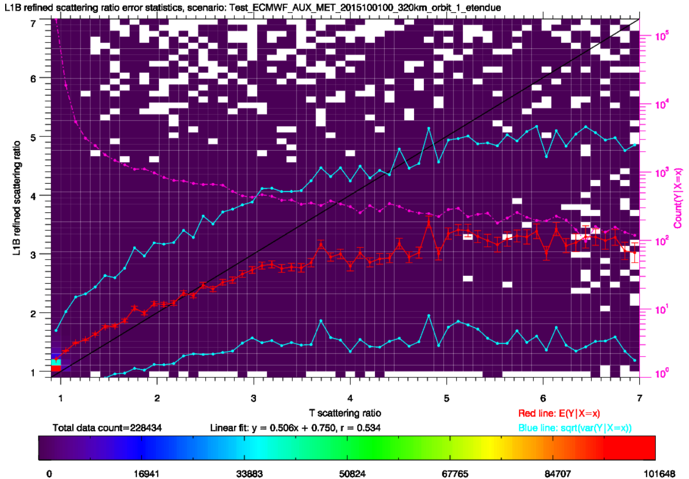
Figure 12. Comparison of the L1B refined scattering ratio to the “truth” (T) scattering ratio for the ECMWF derived cloudy scenario (red line). Pink line: number of observations with a given true or estimated scattering ratio. Black line: 1:1 comparison. Blue lines: 1 sigma standard deviation. A positive bias in the L1B SR is evident for SR < 2.3 and a negative bias for SR > 2.3 . The bias at small SR is more a concern for L2B classification.
