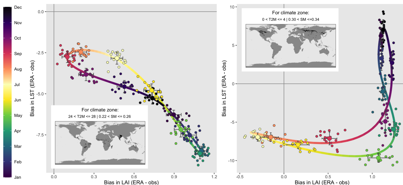
Figure 3. Diagnostic plots illustrating the hysteretic behaviour between the biases in LAI and the biases in LST for two different climate zones. The biases are always defined as ERA5L variables minus the values from reference observational datasets. The small individual points represent monthly values within the entire period 2003-2018. The larger points represent the inter-annual mean values for each month (and the error bars represent one standard deviation). The continuous line is obtained from a harmonic fit.
