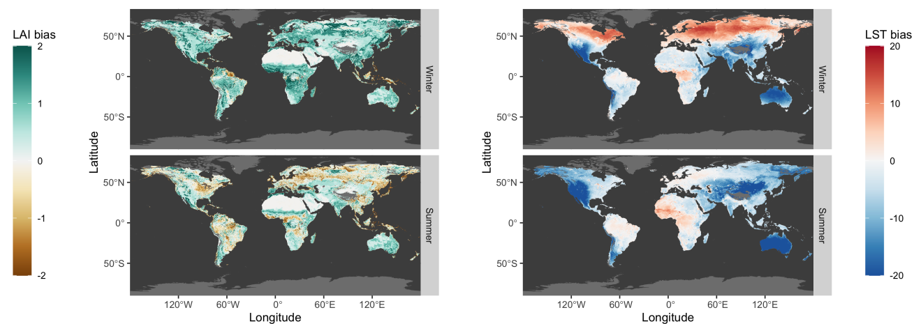
Figure 2. Overview of the mean biases in LAI and LST between ERA5L and observations (ERA - obs) over the climatological period from 2003 to 2018. The panels represent composite maps for which the seasonalities of both Northern and Southern Hemispheres are aligned: winter maps consist of data for January in northern latitudes and July in southern latitudes, while summer maps combine July values in the North with January values in the South.
