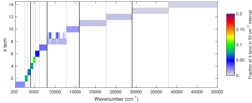
Illustration of the parts of the shortwave spectrum that contribute to each k term of the limited-area-nwp-narrow-14 model.
