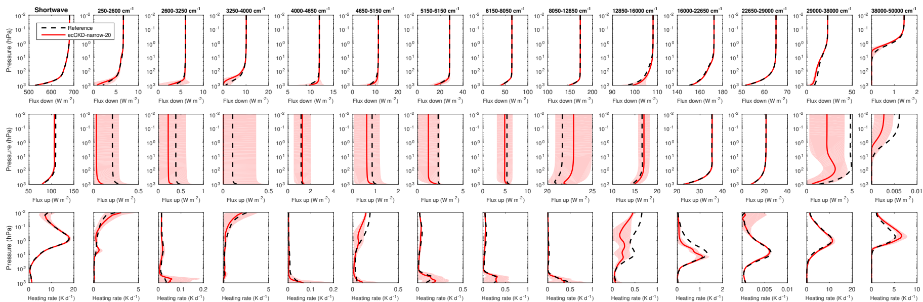
Evaluation of irradiances and heating rates for the broadband (leftmost column of panels) and the 13 narrow shortwave bands (other panels) of the limited-area-nwp-narrow-20 CKD model. The black dashed and red solid lines correspond to the average of the 50 profiles for the “present-day” scenario, while the shaded regions encompass 95% of the error.
