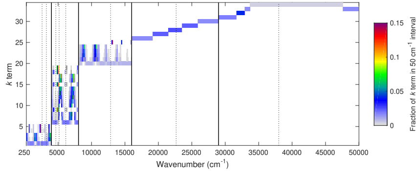
Illustration of the parts of the shortwave spectrum that contribute to each k term of the limited-area-nwp-wide-34 model.
