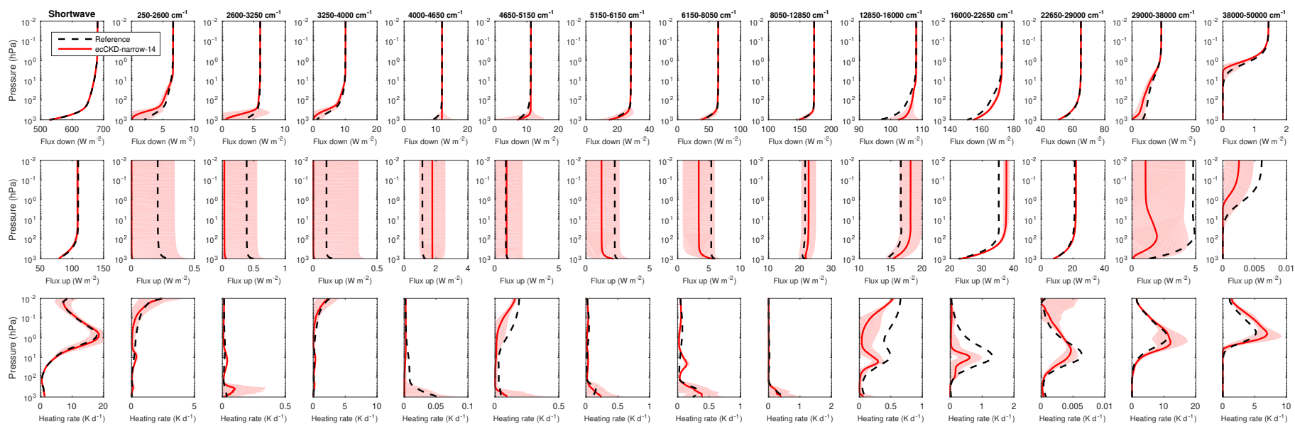
Evaluation of irradiances and heating rates for the broadband (leftmost column of panels) and the 13 narrow shortwave bands (other panels) of the limited-area-nwp-narrow-14 CKD model. The black dashed and red solid lines correspond to the average of the 50 profiles for the “present-day” scenario, while the shaded regions encompass 95% of the error.
