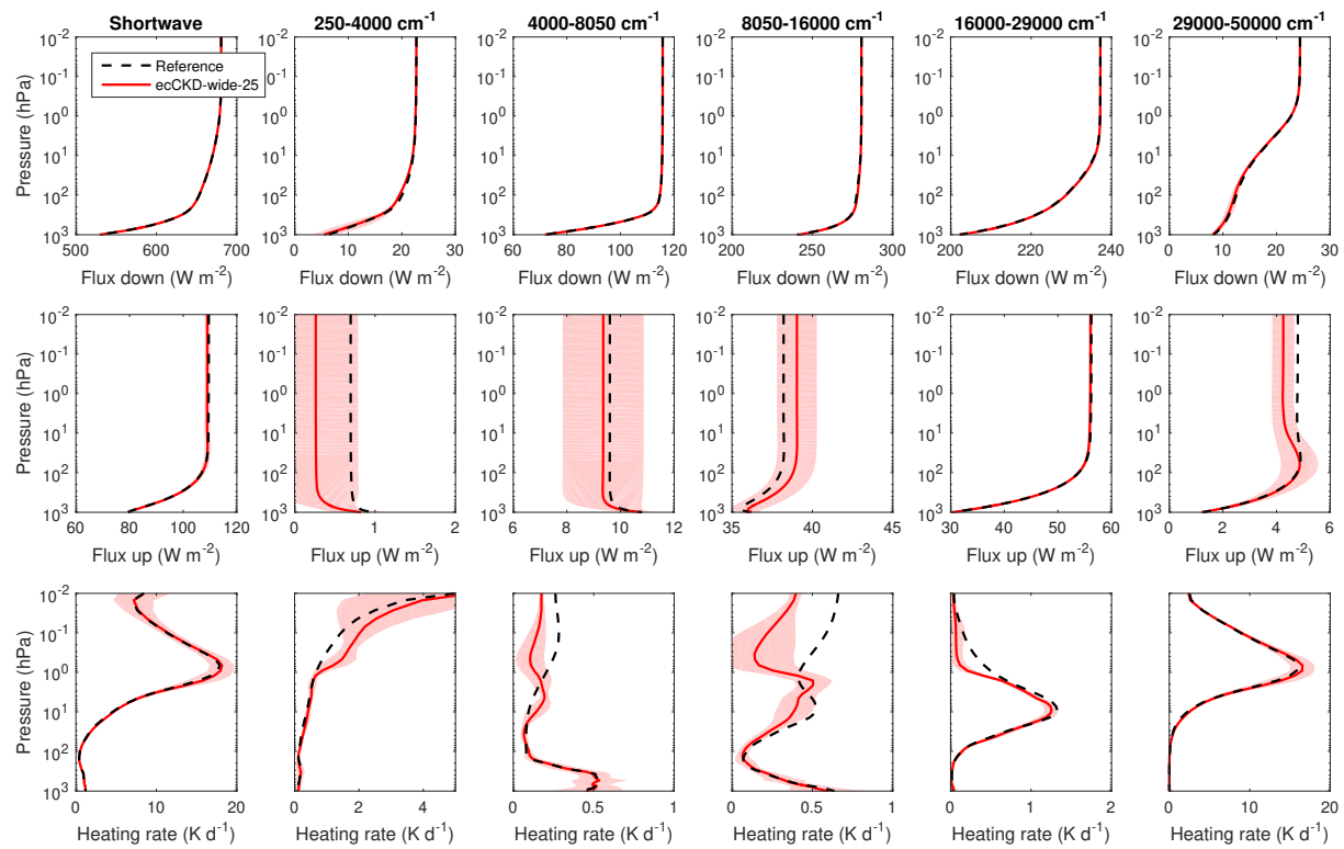
Evaluation of irradiances and heating rates for the broadband (leftmost column of panels) and the 5 wide shortwave bands (other panels) of the limited-area-nwp-wide-25 CKD model. The black dashed and red solid lines correspond to the average of the 50 profiles for the “present-day” scenario, while the shaded regions encompass 95% of the error.
