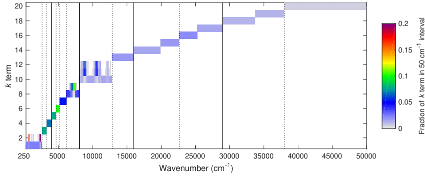
Illustration of the parts of the shortwave spectrum that contribute to each k term of the limited-area-nwp-narrow-20 model.
