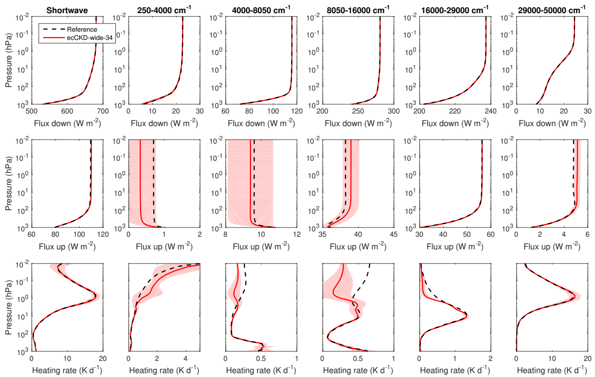
Evaluation of irradiances and heating rates for the broadband (leftmost column of panels) and the 5 wide shortwave bands (other panels) of the limited-area-nwp-wide-34 CKD model. The black dashed and red solid lines correspond to the average of the 50 profiles for the “present-day” scenario, while the shaded regions encompass 95% of the error.
