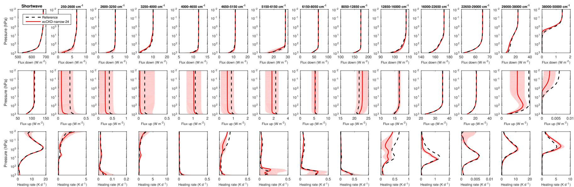
Evaluation of irradiances and heating rates for the broadband (leftmost column of panels) and the 13 narrow shortwave bands (other panels) of the limited-area-nwp-narrow-24 CKD model. The black dashed and red solid lines correspond to the average of the 50 profiles for the “present-day” scenario, while the shaded regions encompass 95% of the error.
