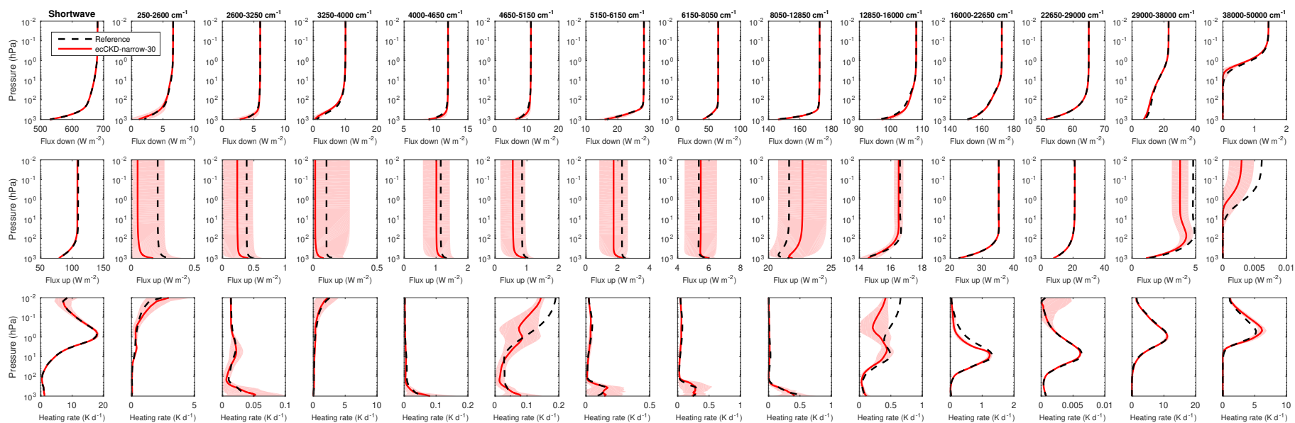
Evaluation of irradiances and heating rates for the broadband (leftmost column of panels) and the 13 narrow shortwave bands (other panels) of the limited-area-nwp-narrow-30 CKD model. The black dashed and red solid lines correspond to the average of the 50 profiles for the “present-day” scenario, while the shaded regions encompass 95% of the error.
