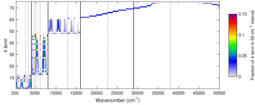
Illustration of the parts of the shortwave spectrum that contribute to each k term of the limited-area-nwp-wide-75 model.
