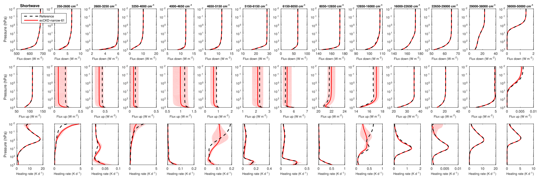
Evaluation of irradiances and heating rates for the broadband (leftmost column of panels) and the 13 narrow shortwave bands (other panels) of the limited-area-nwp-narrow-61 CKD model. The black dashed and red solid lines correspond to the average of the 50 profiles for the “present-day” scenario, while the shaded regions encompass 95% of the error.
