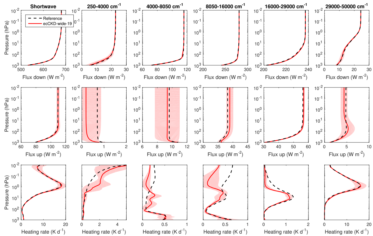
Evaluation of irradiances and heating rates for the broadband (leftmost column of panels) and the 5 wide shortwave bands (other panels) of the limited-area-nwp-wide-19 CKD model. The black dashed and red solid lines correspond to the average of the 50 profiles for the “present-day” scenario, while the shaded regions encompass 95% of the error.
