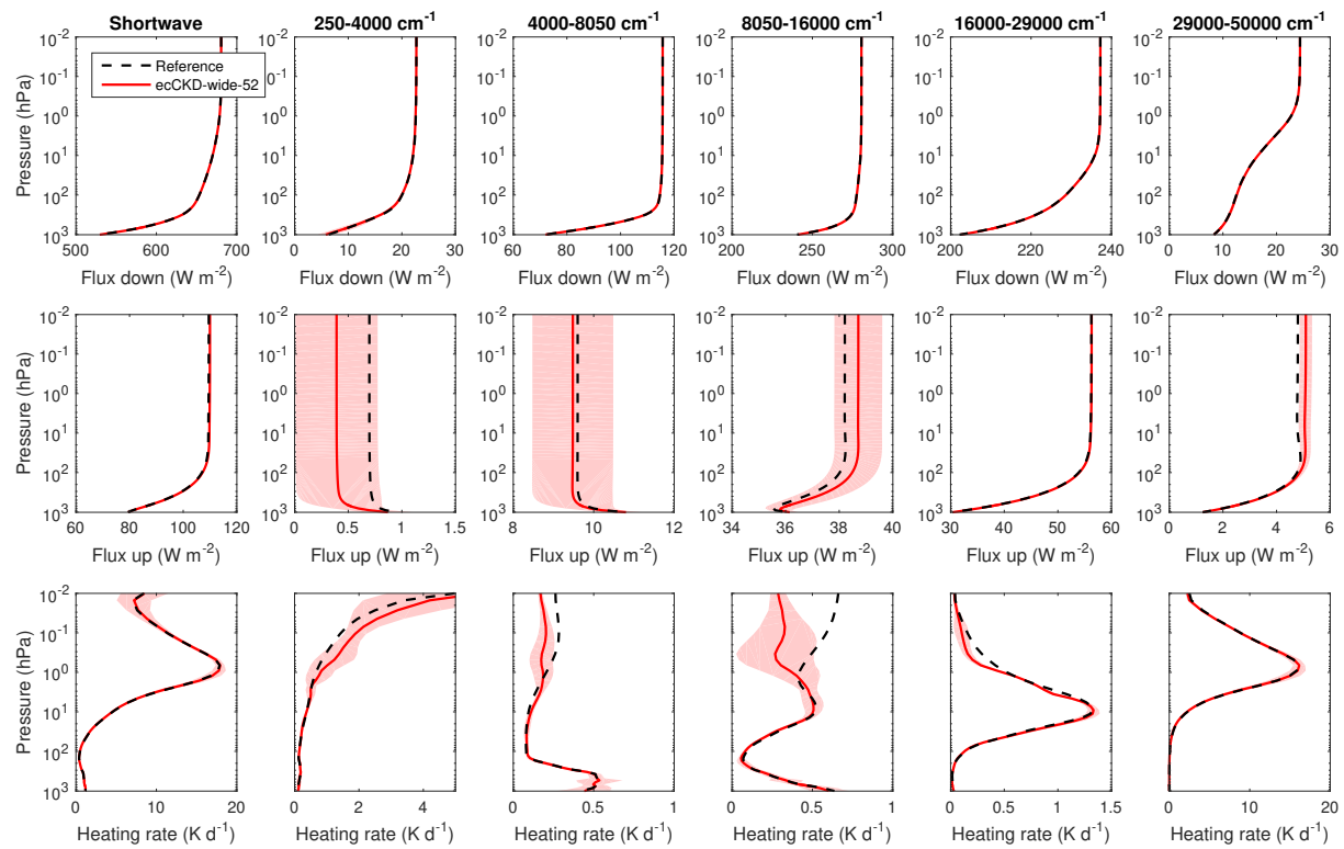
Evaluation of irradiances and heating rates for the broadband (leftmost column of panels) and the 5 wide shortwave bands (other panels) of the limited-area-nwp-wide-52 CKD model. The black dashed and red solid lines correspond to the average of the 50 profiles for the “present-day” scenario, while the shaded regions encompass 95% of the error.
