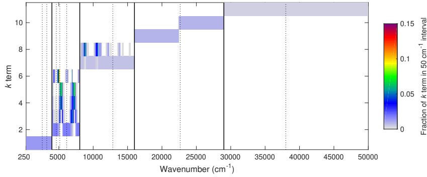
Illustration of the parts of the shortwave spectrum that contribute to each k term of the limited-area-nwp-wide-11 model.
