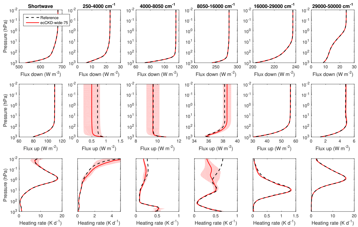
Evaluation of irradiances and heating rates for the broadband (leftmost column of panels) and the 5 wide shortwave bands (other panels) of the limited-area-nwp-wide-75 CKD model. The black dashed and red solid lines correspond to the average of the 50 profiles for the “present-day” scenario, while the shaded regions encompass 95% of the error.
