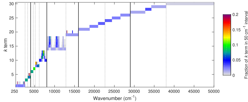
Illustration of the parts of the shortwave spectrum that contribute to each k term of the limited-area-nwp-narrow-30 model.
