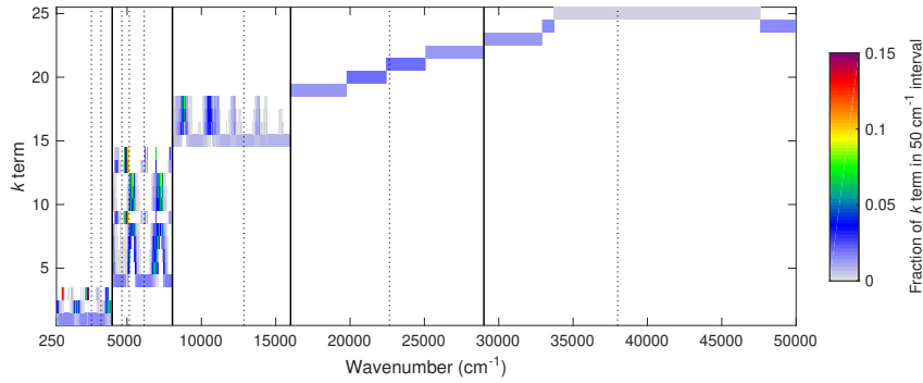
Illustration of the parts of the shortwave spectrum that contribute to each k term of the limited-area-nwp-wide-25 model.
