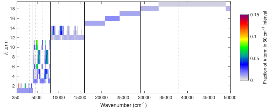
Illustration of the parts of the shortwave spectrum that contribute to each k term of the limited-area-nwp-wide-19 model.
