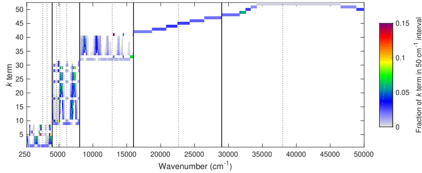
Illustration of the parts of the shortwave spectrum that contribute to each k term of the limited-area-nwp-wide-52 model.
