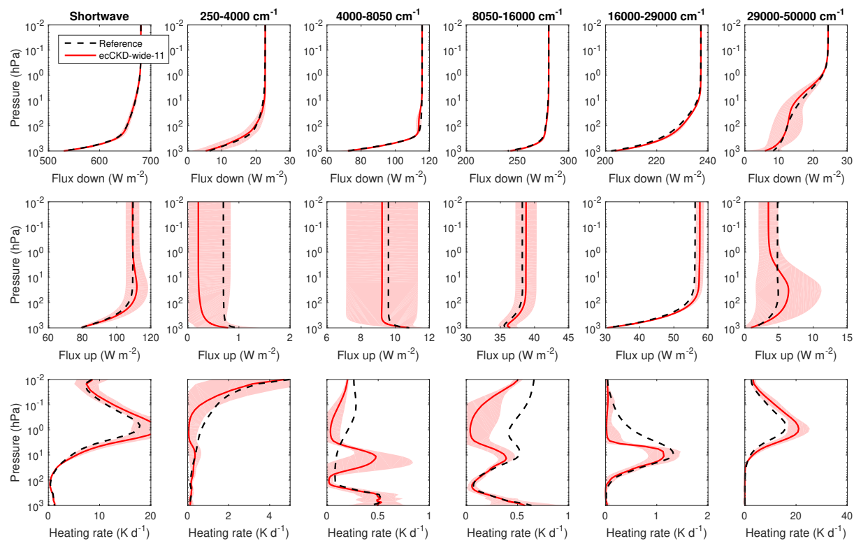
Evaluation of irradiances and heating rates for the broadband (leftmost column of panels) and the 5 wide shortwave bands (other panels) of the limited-area-nwp-wide-11 CKD model. The black dashed and red solid lines correspond to the average of the 50 profiles for the “present-day” scenario, while the shaded regions encompass 95% of the error.
