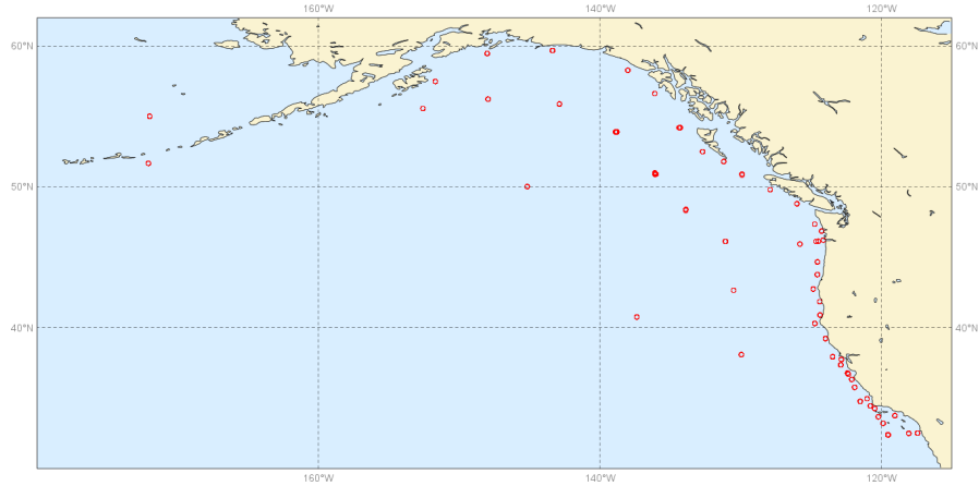
pp1d Scatter index North East Pacific (lat 30 to 62, lon -180 to -115.) Date: 20210301 00UTC to 20210531 12UTC averaged by wave prod. (Mean method, lat)
