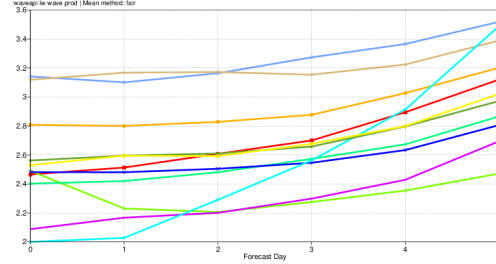
pp1d Root mean square error North East Pacific (lat 30 to 62, lon -180 to -115.) Date: 20210301 00UTC to 20210531 12UTC averaged by wave prod. (Mean method, lat)
