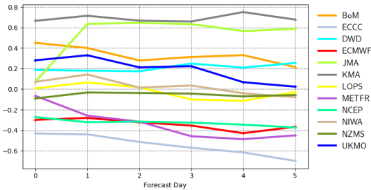
Mean error | pp1d | Eastern Australia and New Zealand 20230301 00z to 20230531 00z | waveapi lw wave prod 00z mean_fair
