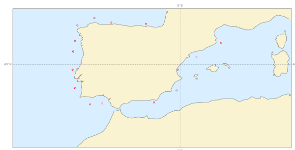
Scatter index | pp1d | SW Europe 20230301 00z to 20230531 00z | waveapi lw wave prod 00z mean_fair
