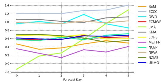
Mean error | pp1d | South Southwestern Australia 20230301 00z to 20230531 00z | waveapi lw wave prod 00z mean_fair
