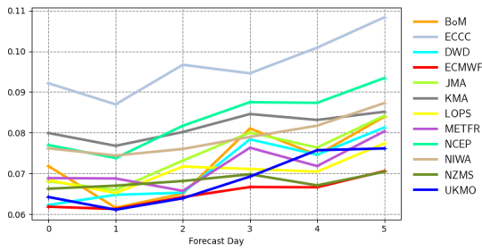
Scatter index | pp1d | South Southwestern Australia 20230301 00z to 20230531 00z | waveapi lw wave prod 00z mean_fair
