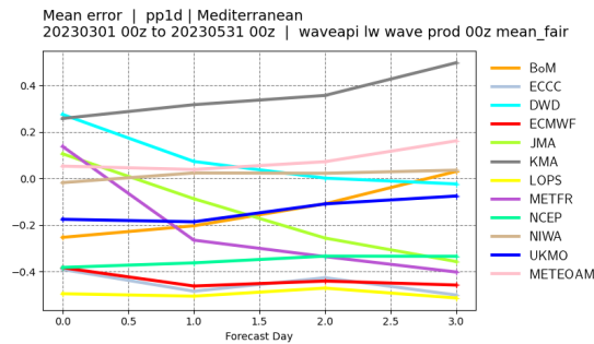
Mediterranean Sea. Top panel: observation distribution. Middle left panel: Forecast scatter index (standard deviation of the difference normalised by the mean of the observations). Middle right panel: Forecast root mean square error (RMSE). Bottom panel: forecast mean error (bias).
