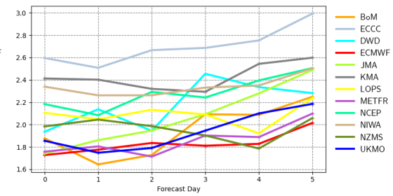
Root mean square error | pp1d | South Southwestern Australia 20230301 00z to 20230531 00z | waveapi lw wave prod 00z mean_fair
