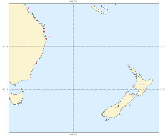
Scatter index | pp1d | Eastern Australia and New Zealand 20230301 00z to 20230531 00z | waveapi lw wave prod 00z mean_fair
