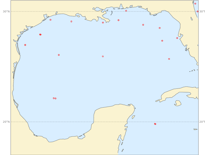
Buoys observations - from 20230301 to 20230531 - (pp1d)
