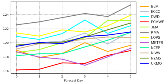
Scatter index | pp1d | Eastern Australia and New Zealand 20230301 00z to 20230531 00z | waveapi lw wave prod 00z mean_fair
