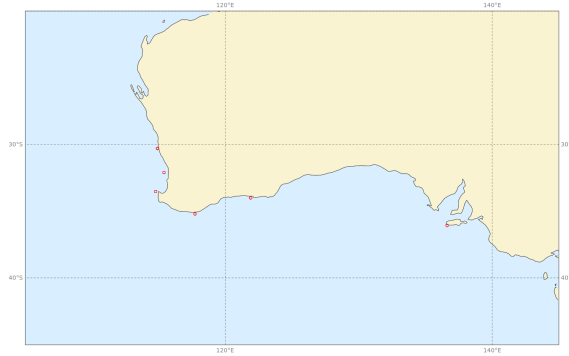
Scatter index | pp1d | South Southwestern Australia 20230301 00z to 20230531 00z | waveapi lw wave prod 00z mean_fair
