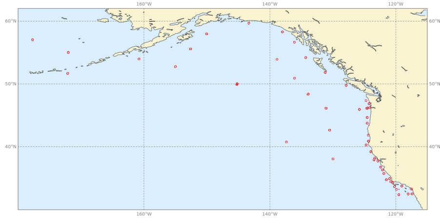
Buoys observations - from 20230301 to 20230531 - (pp1d)
