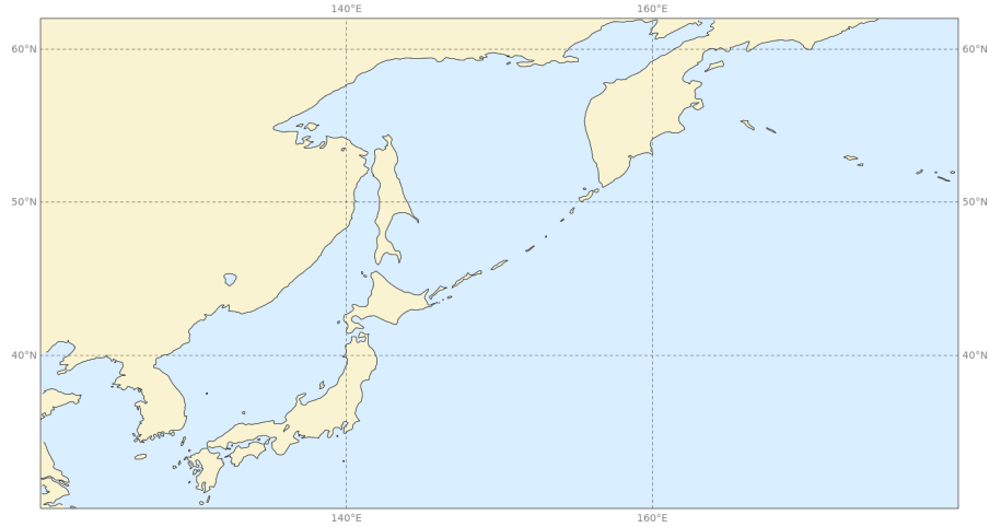
Buoys observations - from 20230301 to 20230531 - (pp1d)
