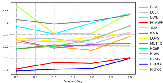
Mean error | pp1d | SW Europe 20230301 00z to 20230531 00z | waveapi lw wave prod 00z mean_fair
