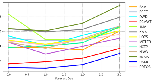
Mean error | pp1d | SW Europe 20230301 00z to 20230531 00z | waveapi lw wave prod 00z mean_fair
