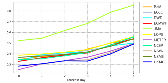
Root mean square error | significant wave height | South Southwestern Austr 20220901 00z to 20221130 12z | waveapi lw wave prod mean_fair
