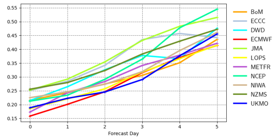
Root mean square error | significant wave height | Gulf of Mexico 20220901 00z to 20221130 12z | waveapi lw wave prod mean_fair
