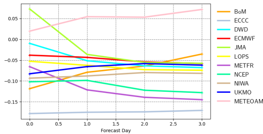
Mean error | significant wave height | Mediterranean 20220901 00z to 20221130 12z | waveapi lw wave prod mean_fair
