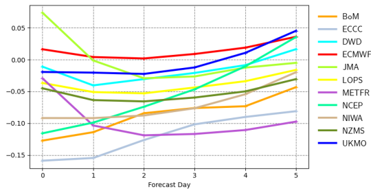
Mean error | significant wave height | Gulf of Mexico 20220901 00z to 20221130 12z | waveapi lw wave prod mean_fair
