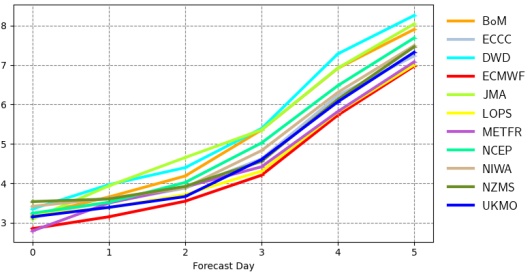
Root mean square error | significant wave height | Europe 20220901 00z to 20221130 12z | waveapi lw wave prod mean_fair
