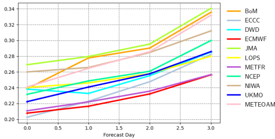
Scatter index | significant wave height | Mediterranean 20220901 00z to 20221130 12z | waveapi lw wave prod mean_fair
