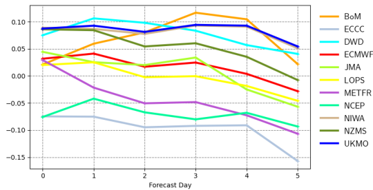
Mean error | significant wave height | Europe 20220901 00z to 20221130 12z | waveapi lw wave prod mean_fair
