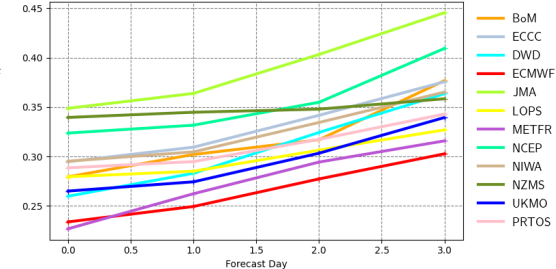
Mean error | significant wave height | SW Europe 20220901 00z to 20221130 12z | waveapi lw wave prod mean_fair
