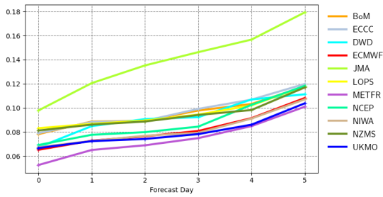
Scatter index | significant wave height | South Southwestern Australia 20220901 00z to 20221130 12z | waveapi lw wave prod mean_fair
