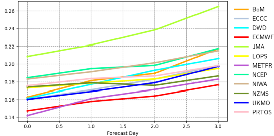
Mean error | significant wave height | SW Europe 20220901 00z to 20221130 12z | waveapi lw wave prod mean_fair
