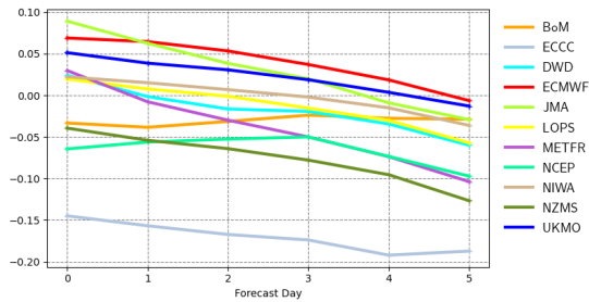
Mean error | significant wave height | North West Atlantic 20220901 00z to 20221130 12z | waveapi lw wave prod mean_fair
