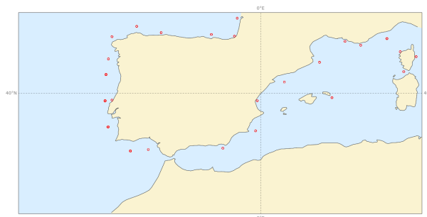
Scatter index | significant wave height | SW Europe 20220901 00z to 20221130 12z | waveapi lw wave prod mean_fair
