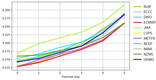
Scatter index | significant wave height | North West Atlantic 20220901 00z to 20221130 12z | waveapi lw wave prod mean_fair
