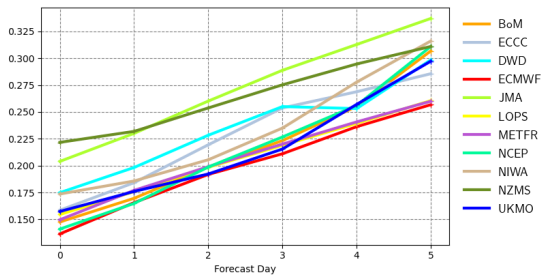
Scatter index | significant wave height | Gulf of Mexico 20220901 00z to 20221130 12z | waveapi lw wave prod mean_fair
