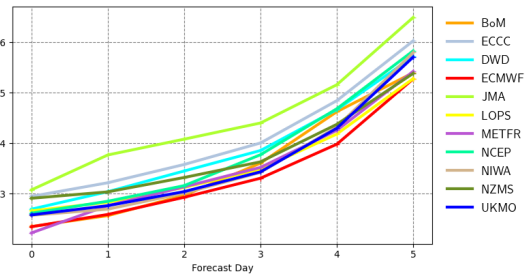
Root mean square error | significant wave height | North West Atlantic 20220901 00z to 20221130 12z | waveapi lw wave prod mean_fair
