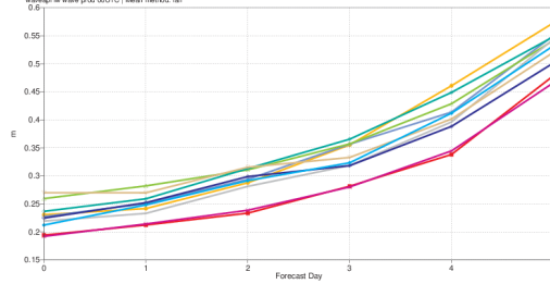
significant wave height Root mean square error Europe (lat. 35.0 to 75.0, lon. -12.5 to 42.5) Date: 20190601 00UTC to 20190831 00UTC Average for wave prod. 00UTC. Mean method. 1st.
