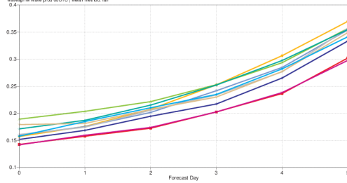
significant wave height Scatter index Europe (lat. 35.0 to 75.0, lon. -12.5 to 42.5) Date: 20190601 00UTC to 20190831 00UTC Average for wave prod. 00UTC. Mean method. 1st.
