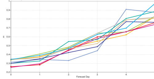
significant wave height Root mean square error North West Pacific (lat 30 to 62, lon 120 to 180) Date: 20190901 00UTC to 20191130 00UTC averaged by wave period (0UTC, 180m method, lat)
