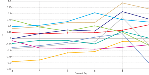
significant wave height Mean error North West Pacific (lat 30 to 62, lon 120 to 180) Date: 20190901 00UTC to 20191130 00UTC averaged by wave period (0UTC, 180m method, lat)
