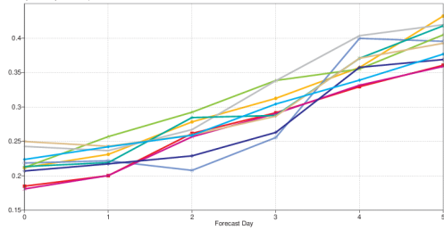
significant wave height Scatter index North West Pacific (lat 30 to 62, lon 120 to 180) Date: 20190901 00UTC to 20191130 00UTC averaged by wave period (0UTC, 180m method, lat)
